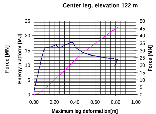
Figure 7 Force-deformation and energy dissipation curves in jacket.
