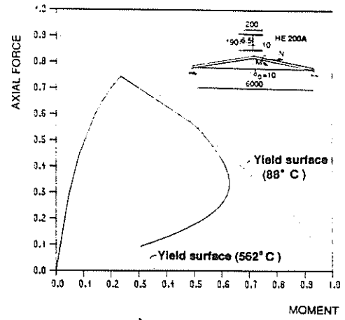
b) Axial force - bending moment interaction
